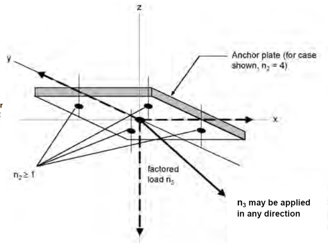
FIGURE 4b—DETAIL A: ANCHORAGE POINT
